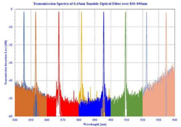
Typical Spectra & Tuning Feature of 0.15nm FWHM Tunable Filter over 830-950nm
