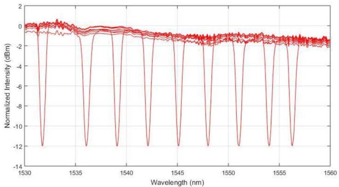
Fig.2. FBG transmission spectra over the tuning range.
