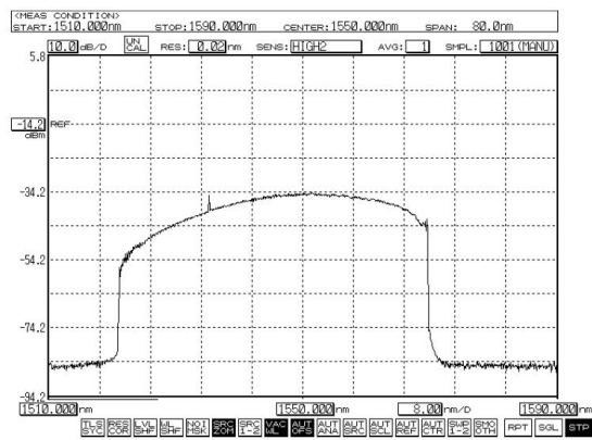
Swept laser spectrum at 1550nm.
