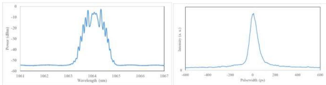
spectrum and pulse shape at 1060 nm
