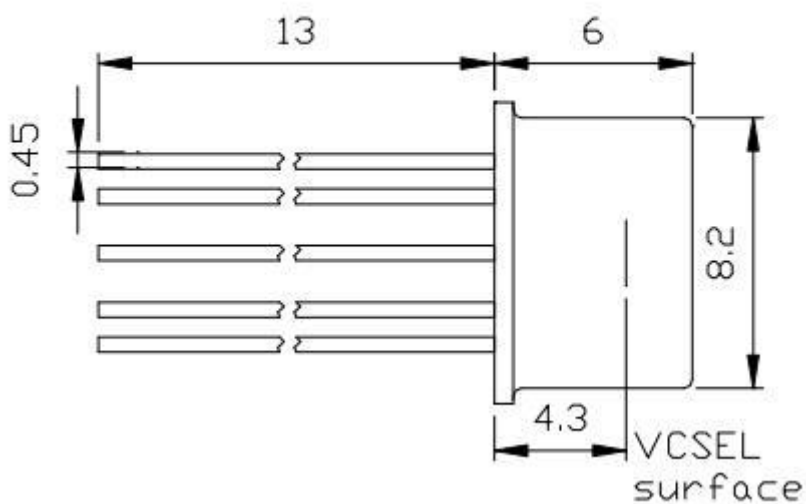
TO dimensions
