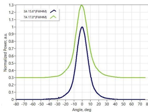
Fast Axis Far Field
