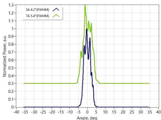
Slow Axis Far Field
