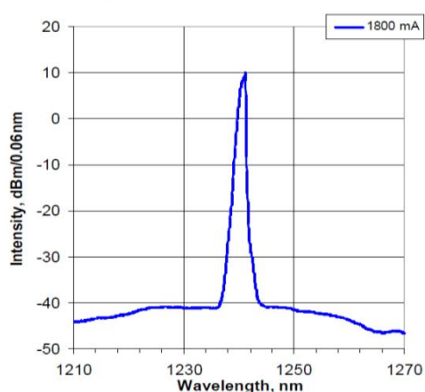
Spectral Characteristics
