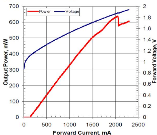
Light-Current-Voltage Characteristics
