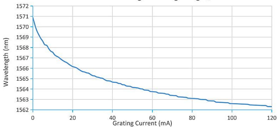
19090101 Wavelength Tuning Range@25°C
