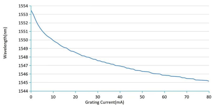
1550nm DBR Wavelength Tuning Range@25°C
