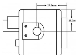
Bottom installation hole diagram
