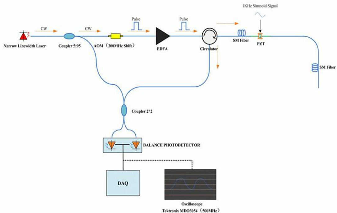
Coherent detection distributed optical fiber sensing
