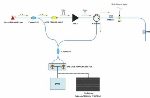
Coherent Detection Distributed Fiber Optic Sensing
