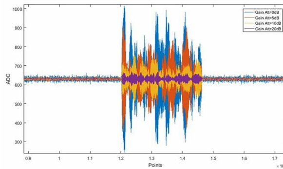
200MHz beat frequency signal (oscilloscope data)
