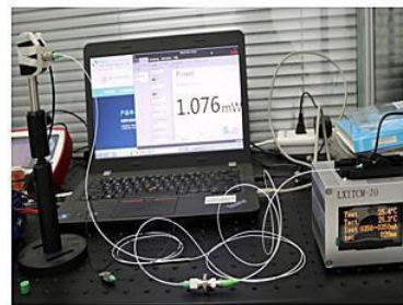
white port@1550nm
