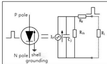
Figure 5 Equivalent circuit
