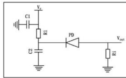
Figure 6 Application circuit
