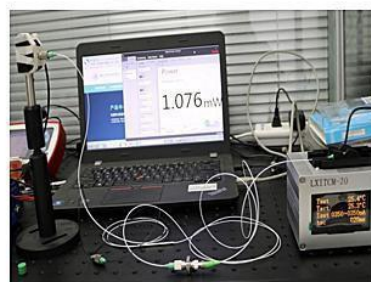
white port@1550nm
