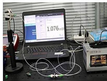
white port@1550nm
