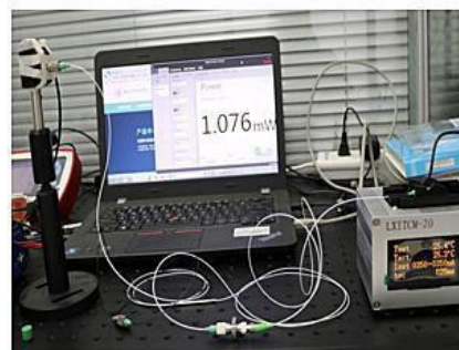
white port@1550nm
