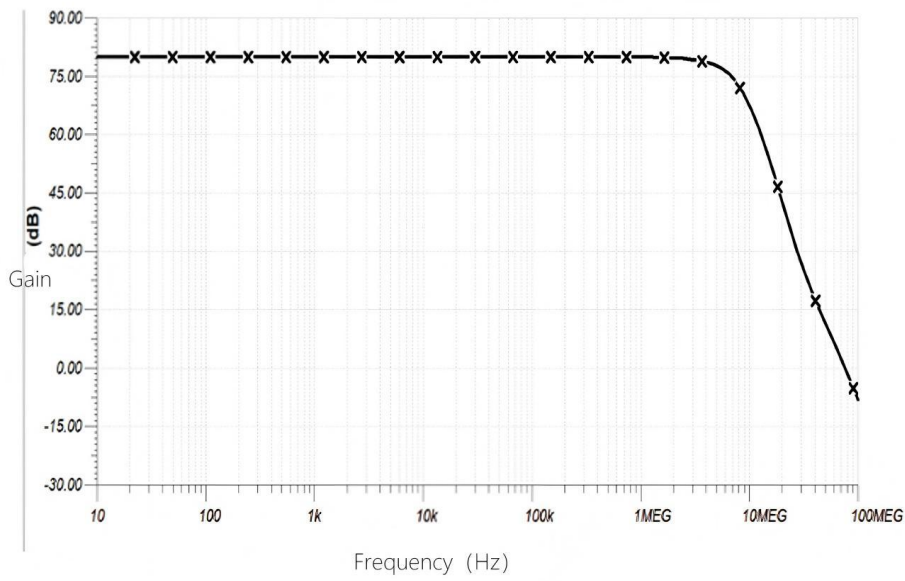
AC transfer characteristics
