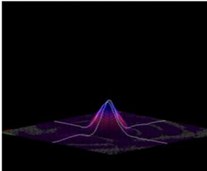
3-D Beam Profile at 1016.0 mm (40.0 in)
