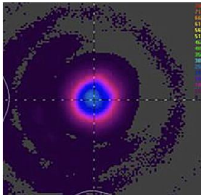
2-D Beam Profile at 1016.0 mm (40.0 in)
