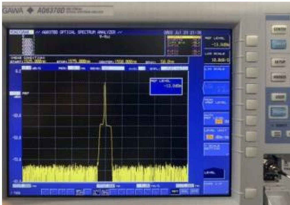
Spectrum test @ 10kHz, 3ns, 100μJ.
