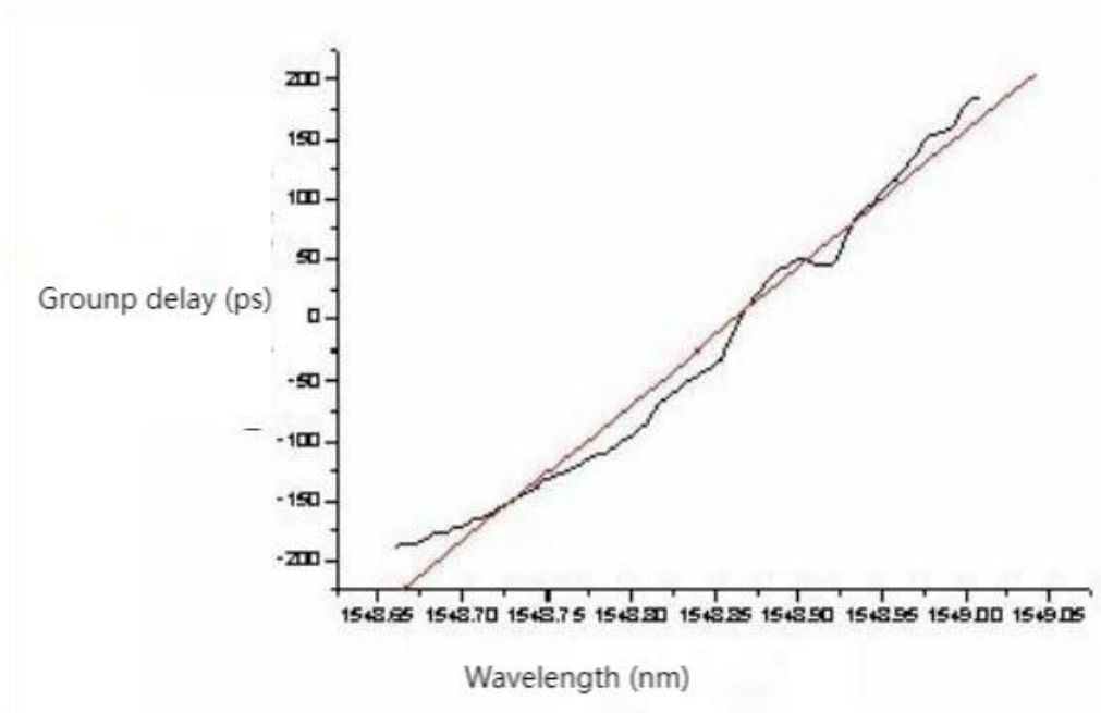
Figure 1: Dispersion curve
