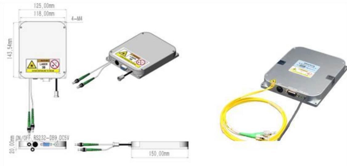
M20 Modular Model and Dimensions
