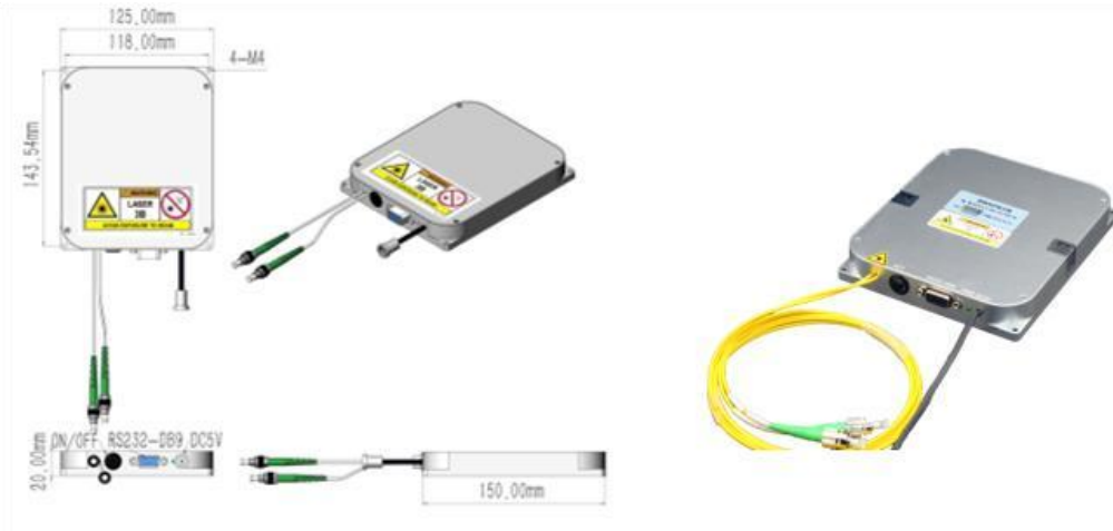
M20 Modular Model and Dimensions
