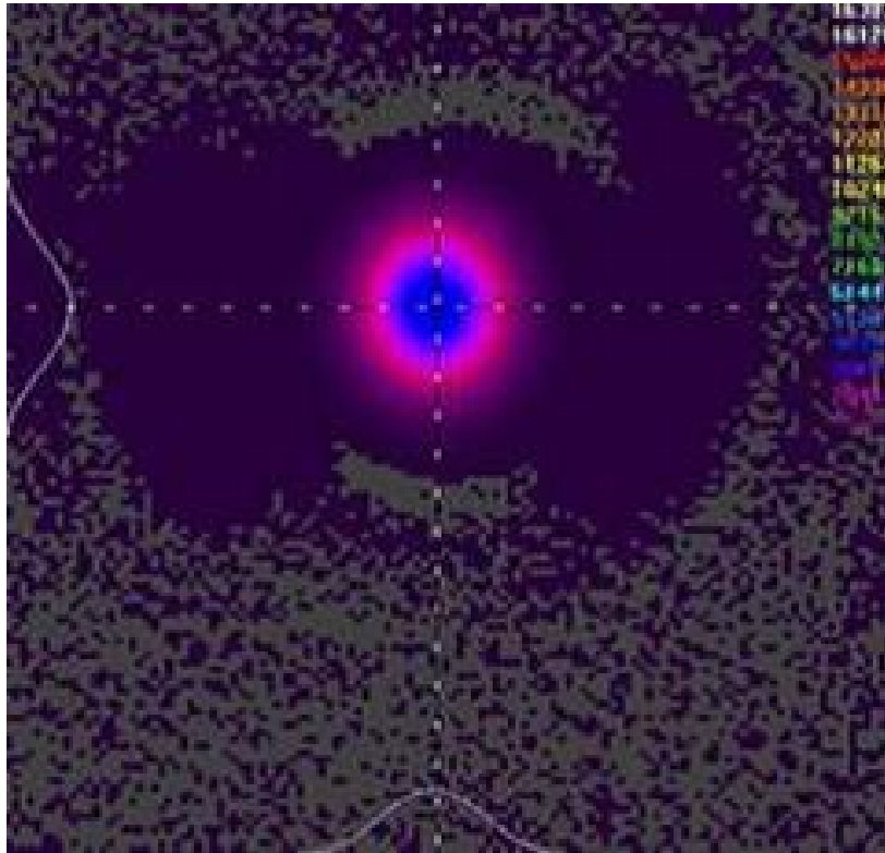
2-D Beam Profile at 1778 mm (70.0 in)
