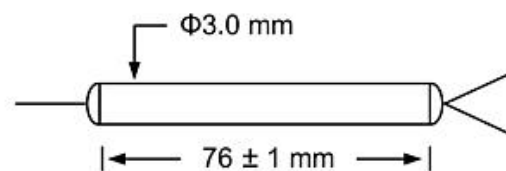
900 μm loose tube
