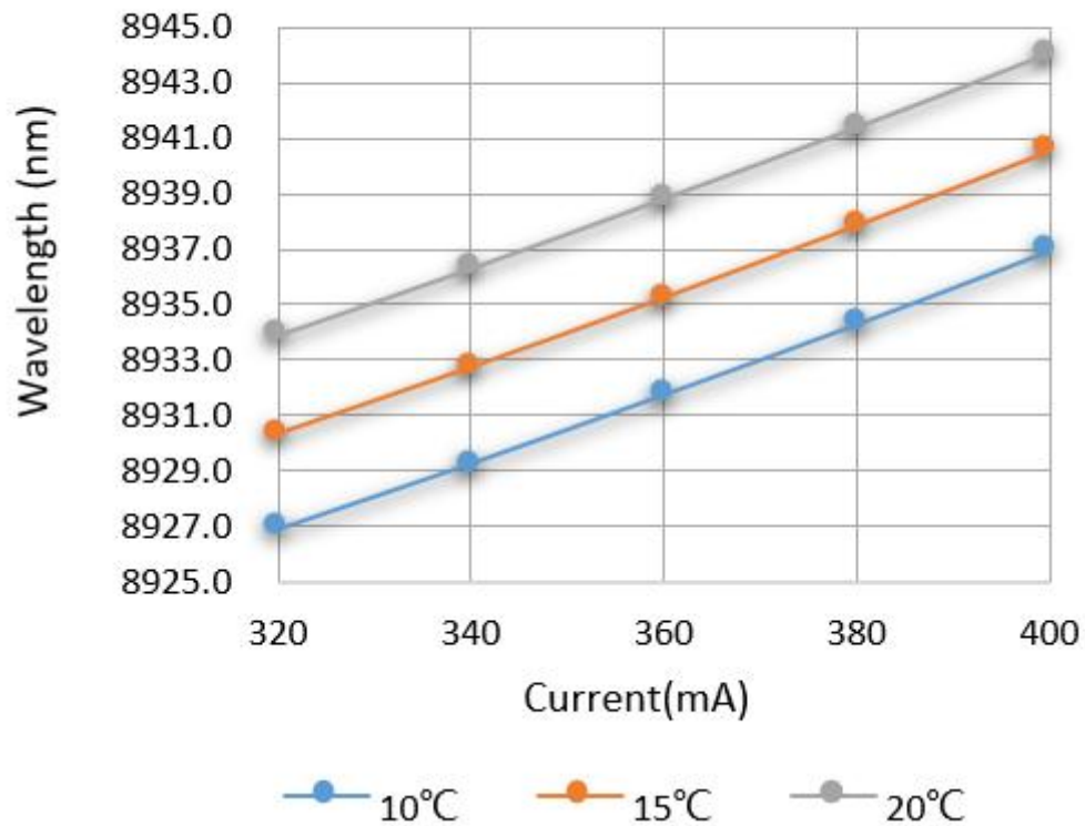
Tuning Characteristics
