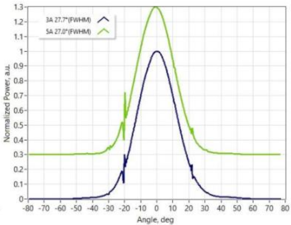
Far-axis far-field
