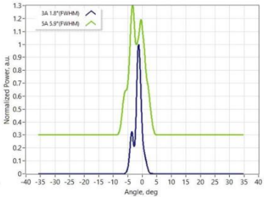
Slow-axis far-field
