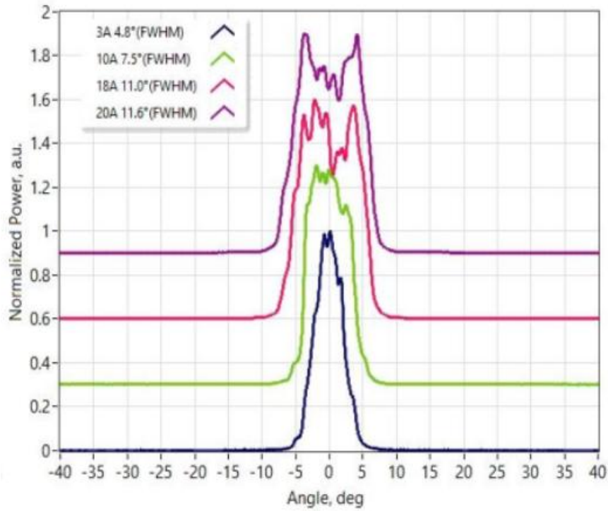
Slow-axis far-field
