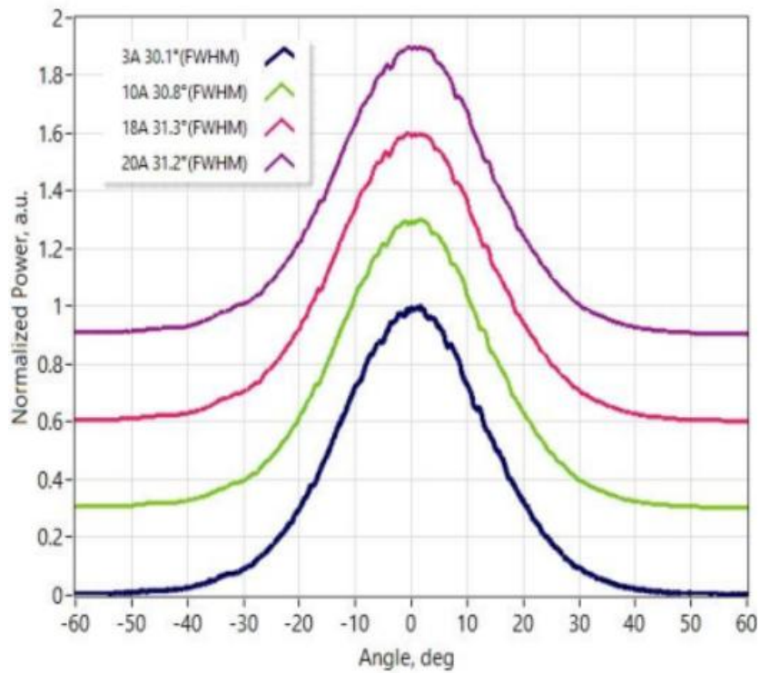
Far-axis far-field
