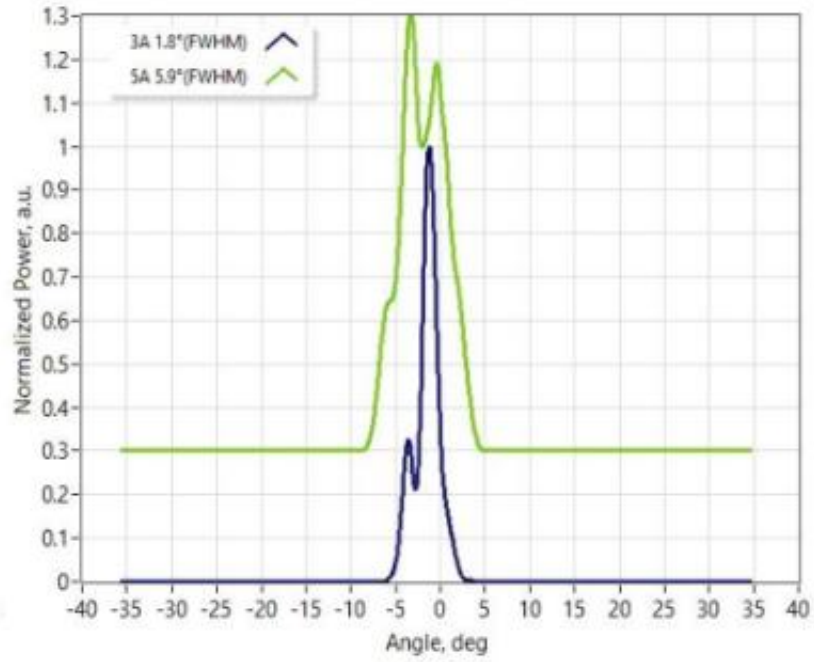
Slow-axis far-field
