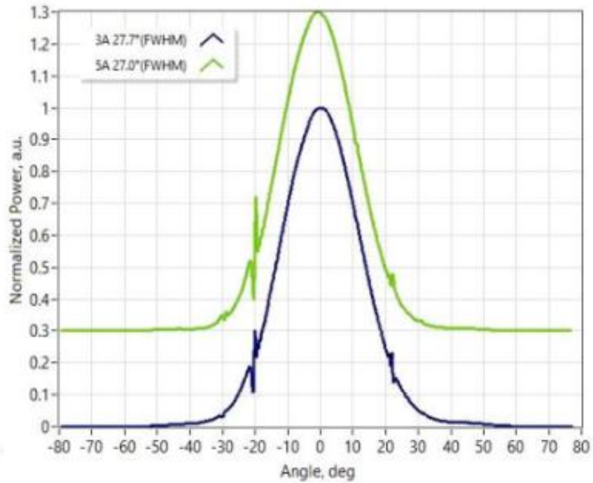
Far-axis far-field
