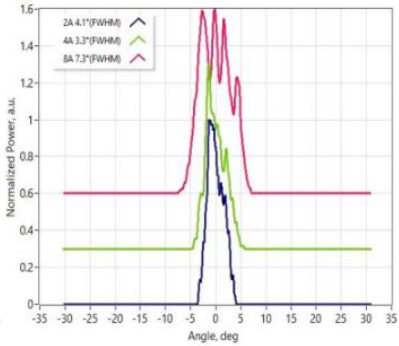
Slow-axis far-field
