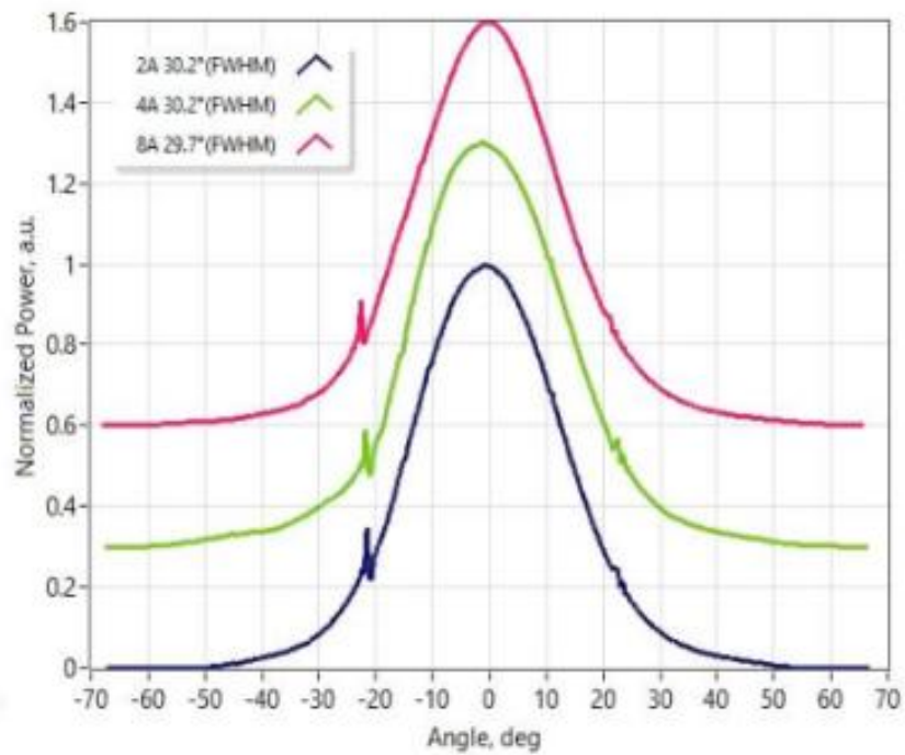
Far-axis far-field
