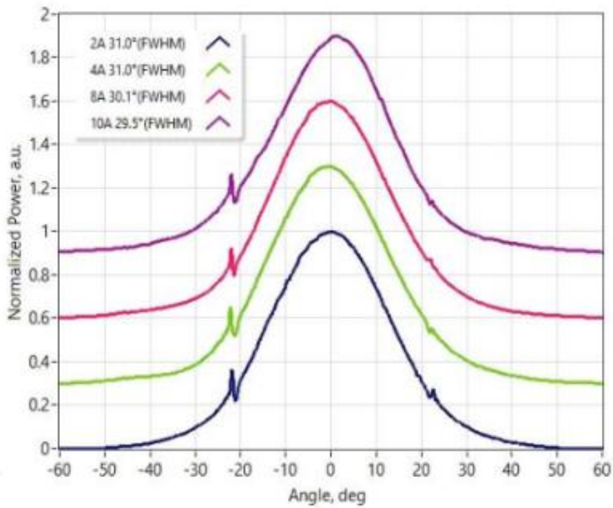
Far-axis far-field
