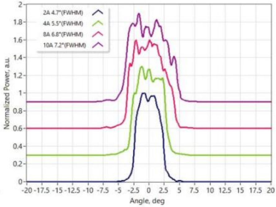
Slow-axis far-field
