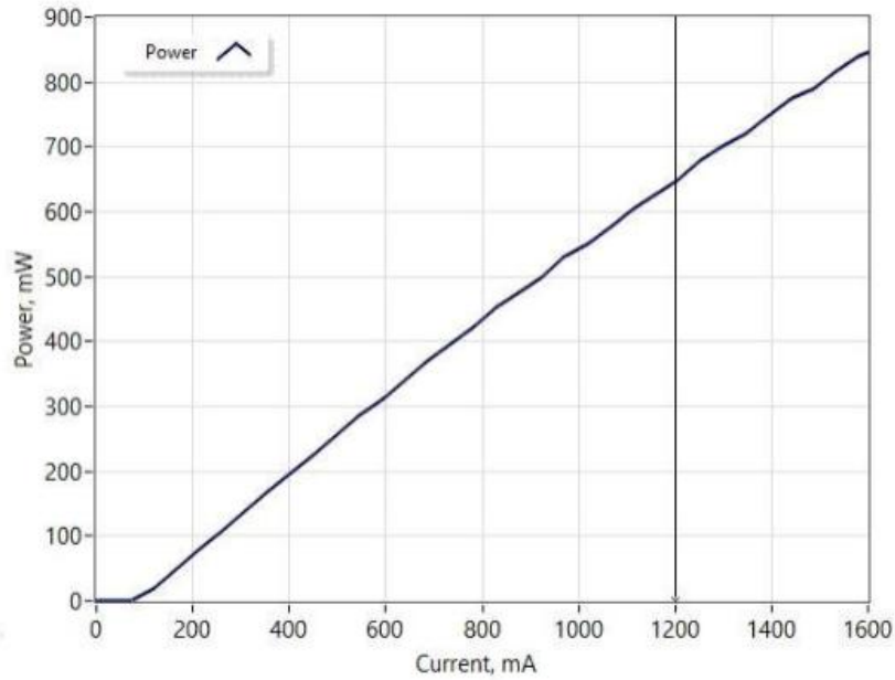
L-I-V characteristic graph
