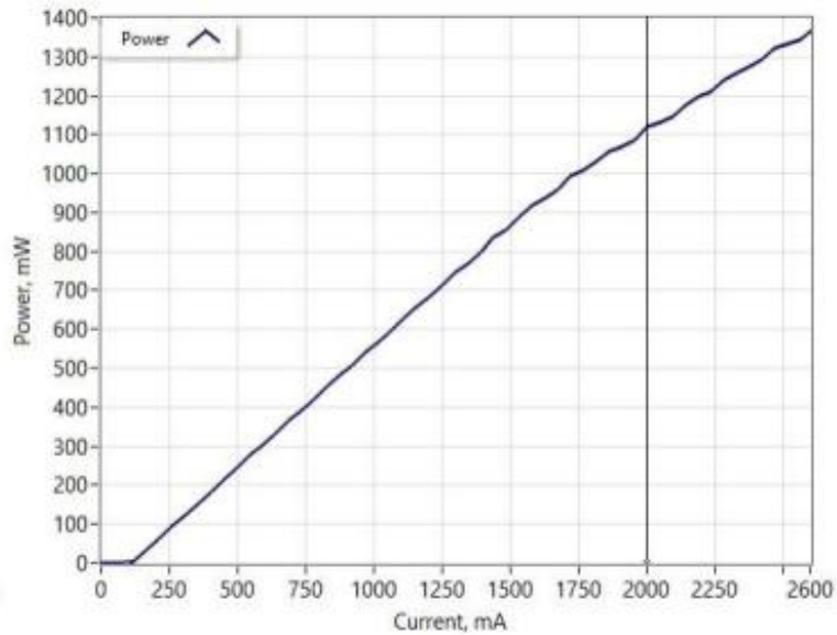
L-I-V characteristic graph
