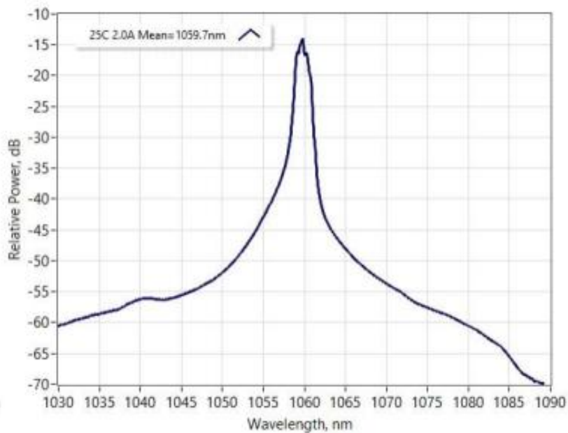
Optical Spectrum (Resolution 200pm)
