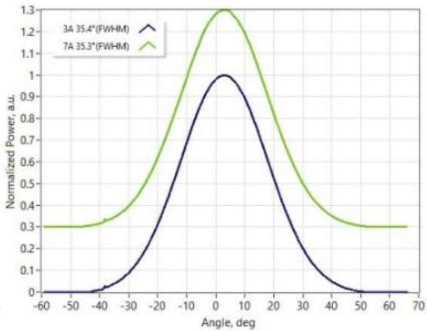
Far-axis far-field
