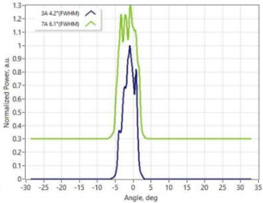
Slow-axis far-field
