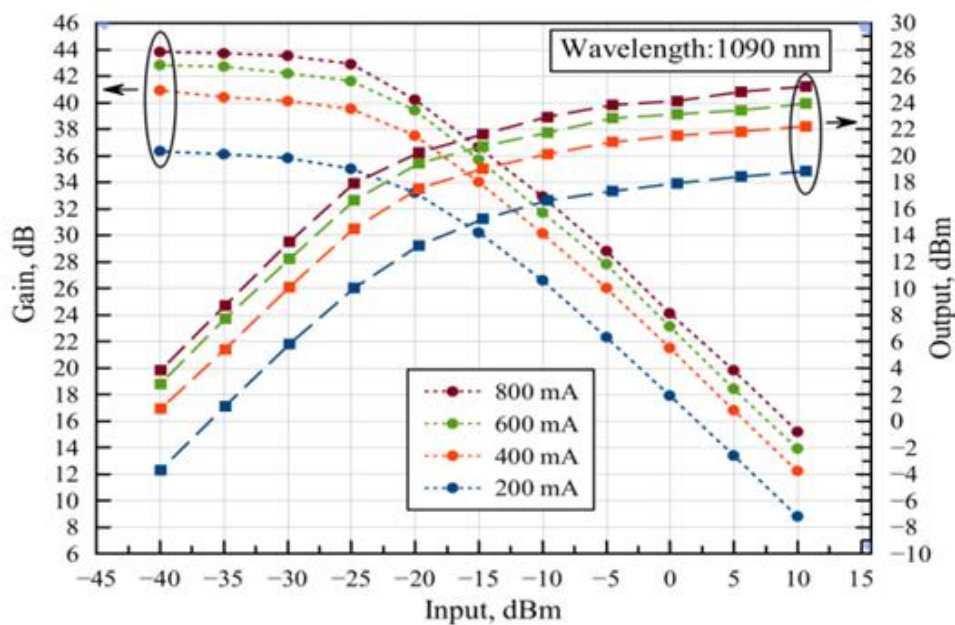
Gain and Output power vs. Input signal
