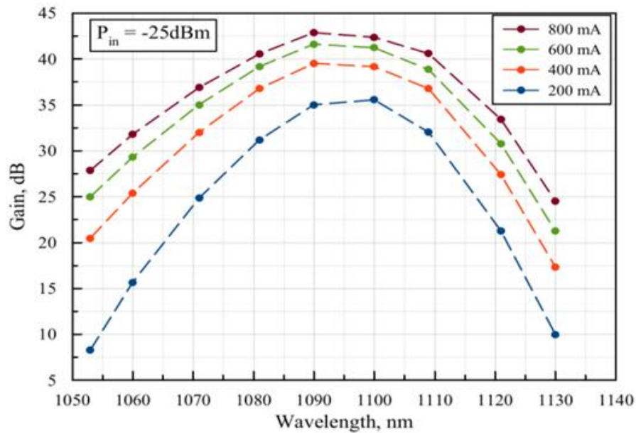
Gain spectra at different currents
