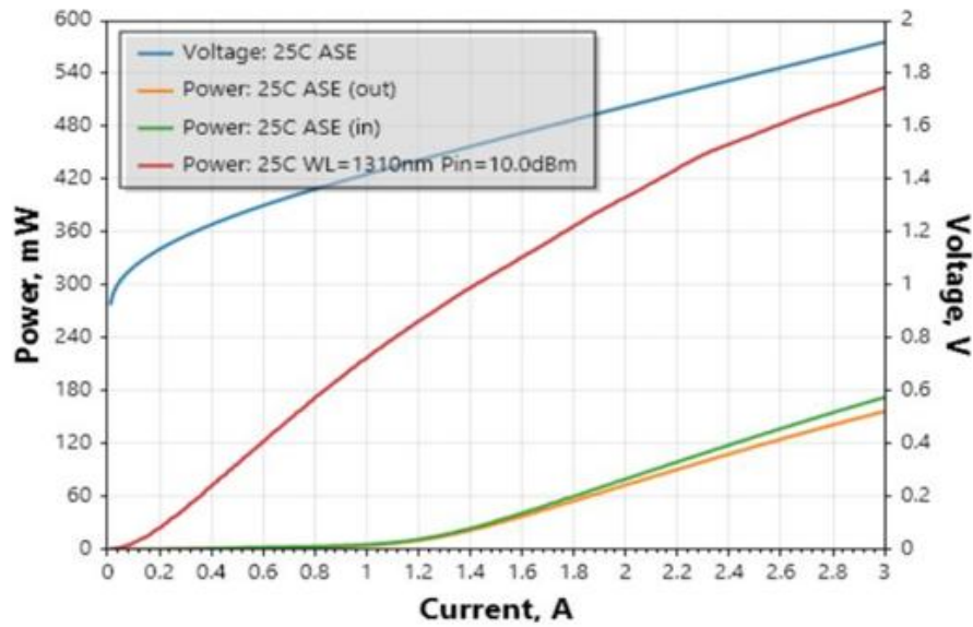
Output Power vs Operating Current
