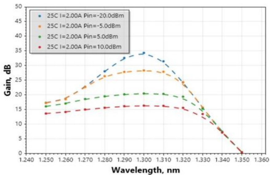
Gain Spectra
