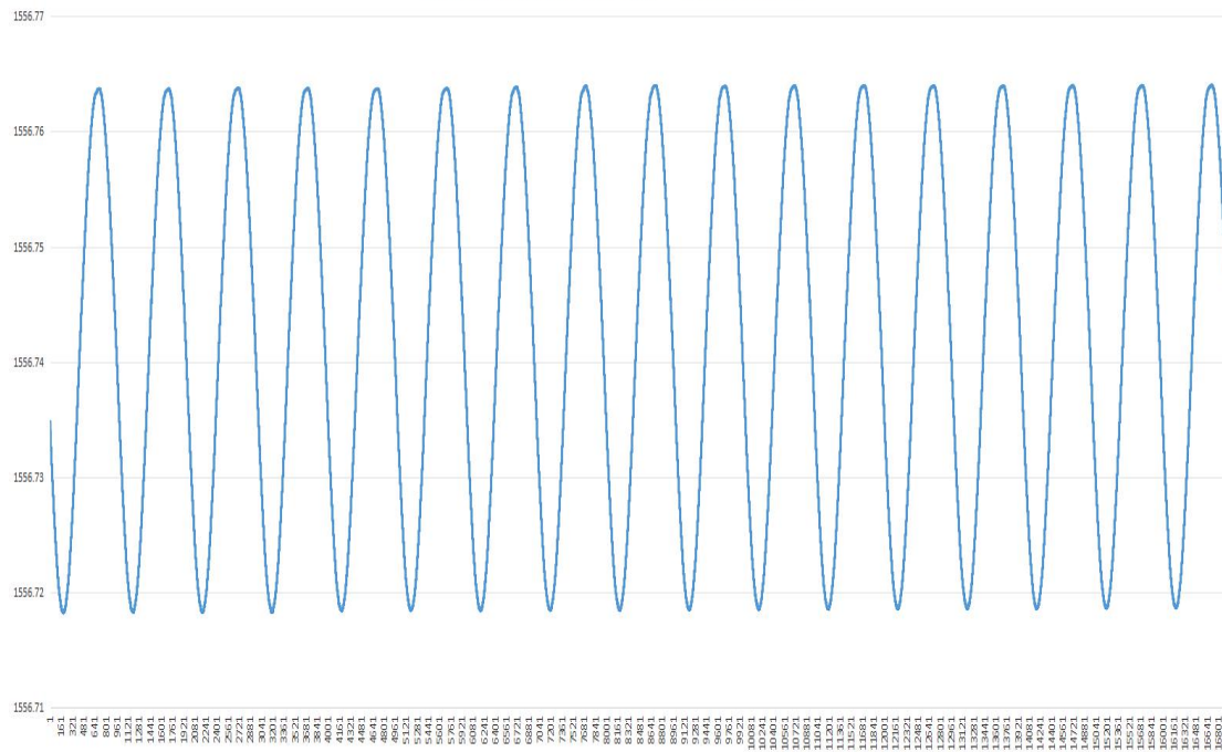
1557nm Narrow Linewidth PZT Laser Mode Hop Free Tuning Range
