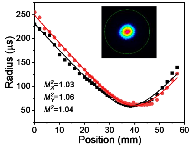
Figure 4. M 2 Test
